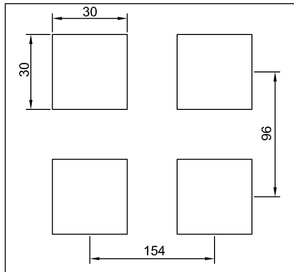
Fundamentplan Fero
